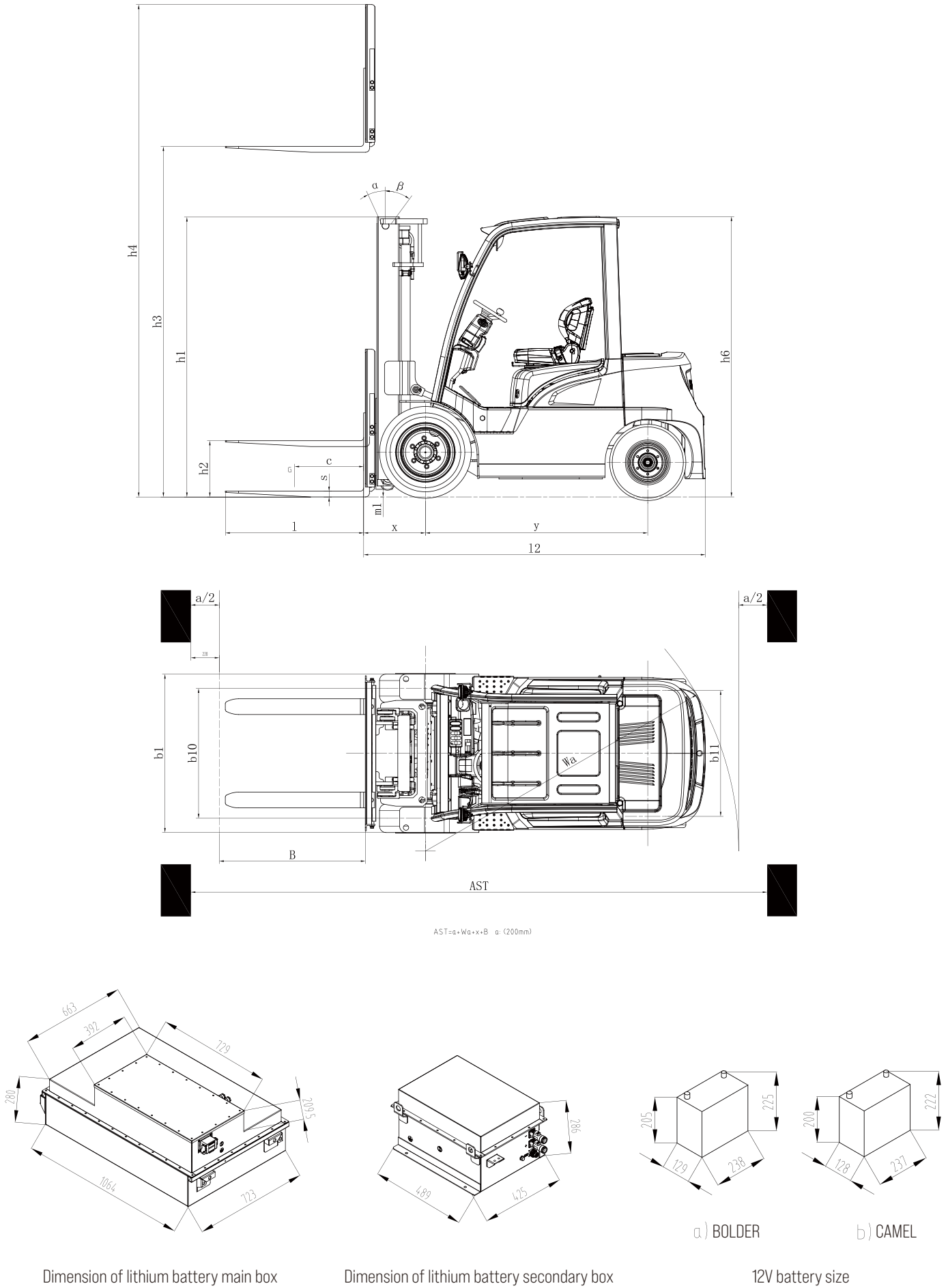
Dimension of lithium battery main box
